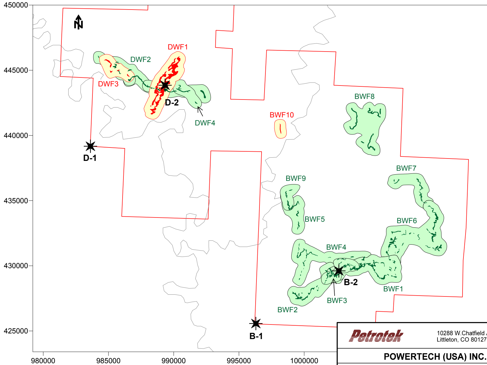
Figure 6-27. Location of Monitor Points Assessment of ISR Effects on Hydraulic Head Dewey-Burdock Project, South Dakota
